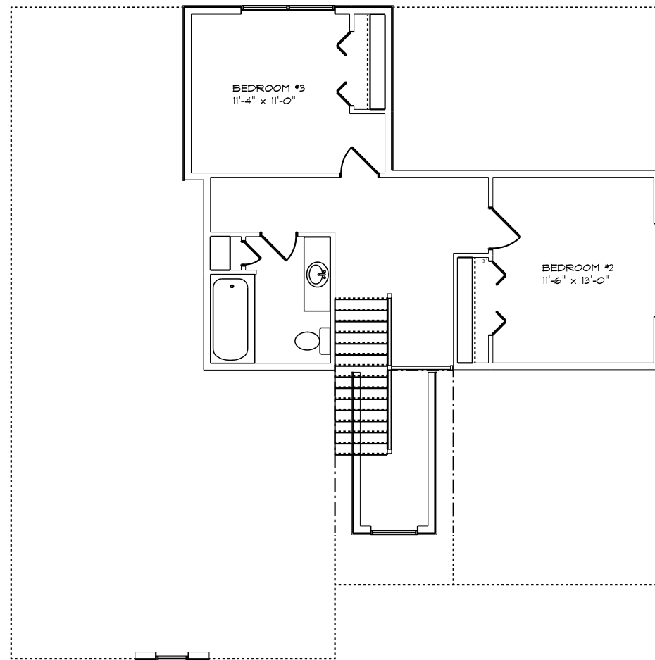
2 nd Floor
