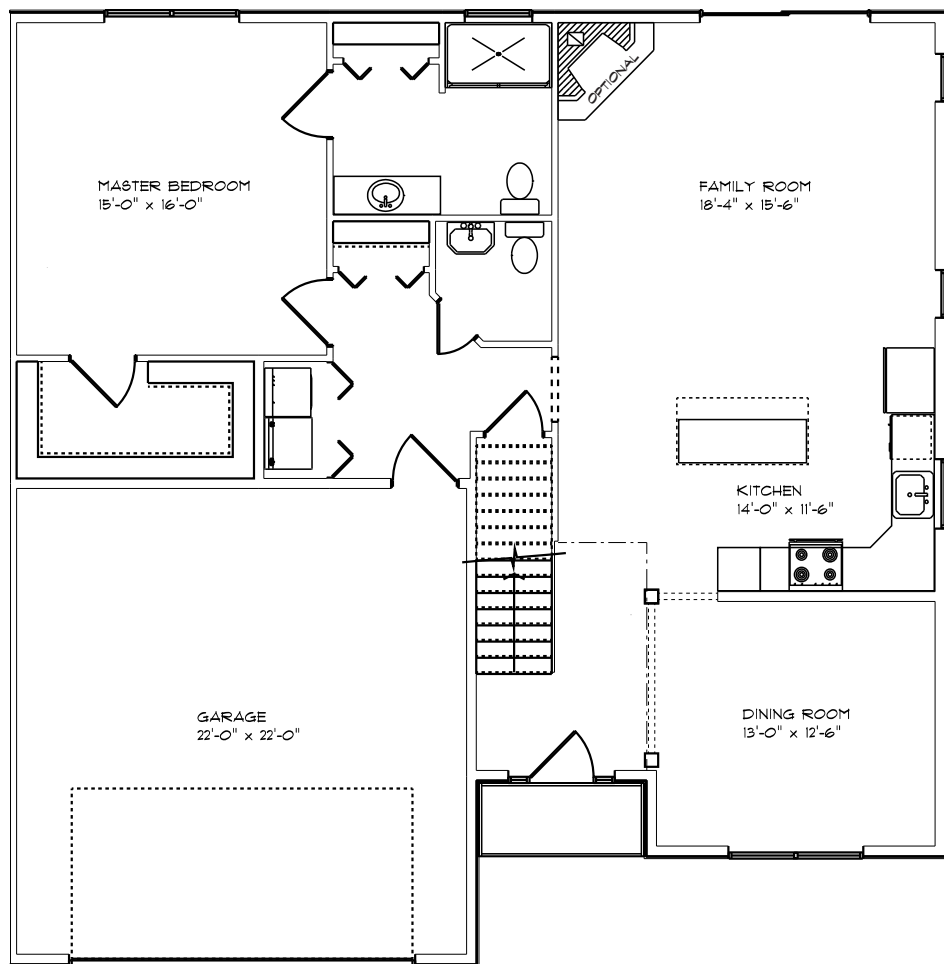
1 st Floor
