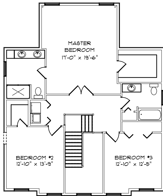
2 nd Floor 1,219 ft 2
