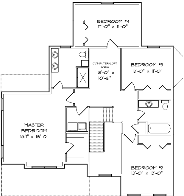
2 nd Floor 1,457 ft 2
